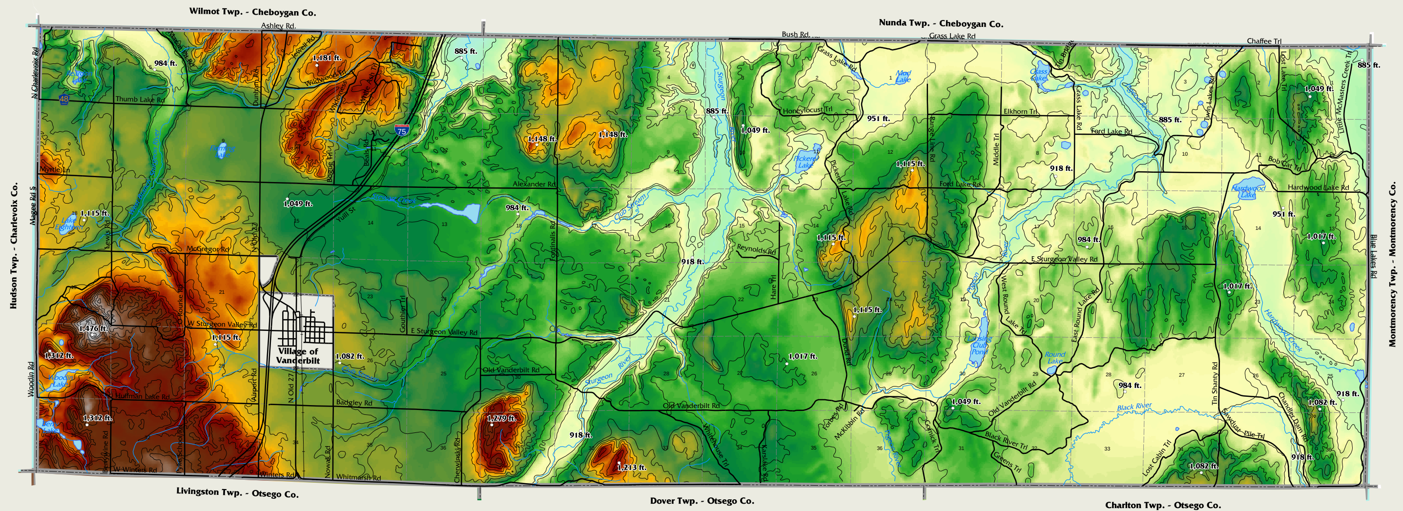
Figure 2 Topography Legend
